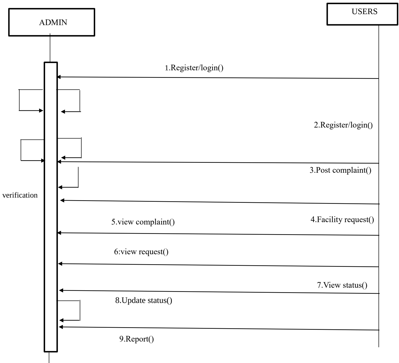
Fig.No.7.1.4. sequence diagram for Grievance Redressal system
