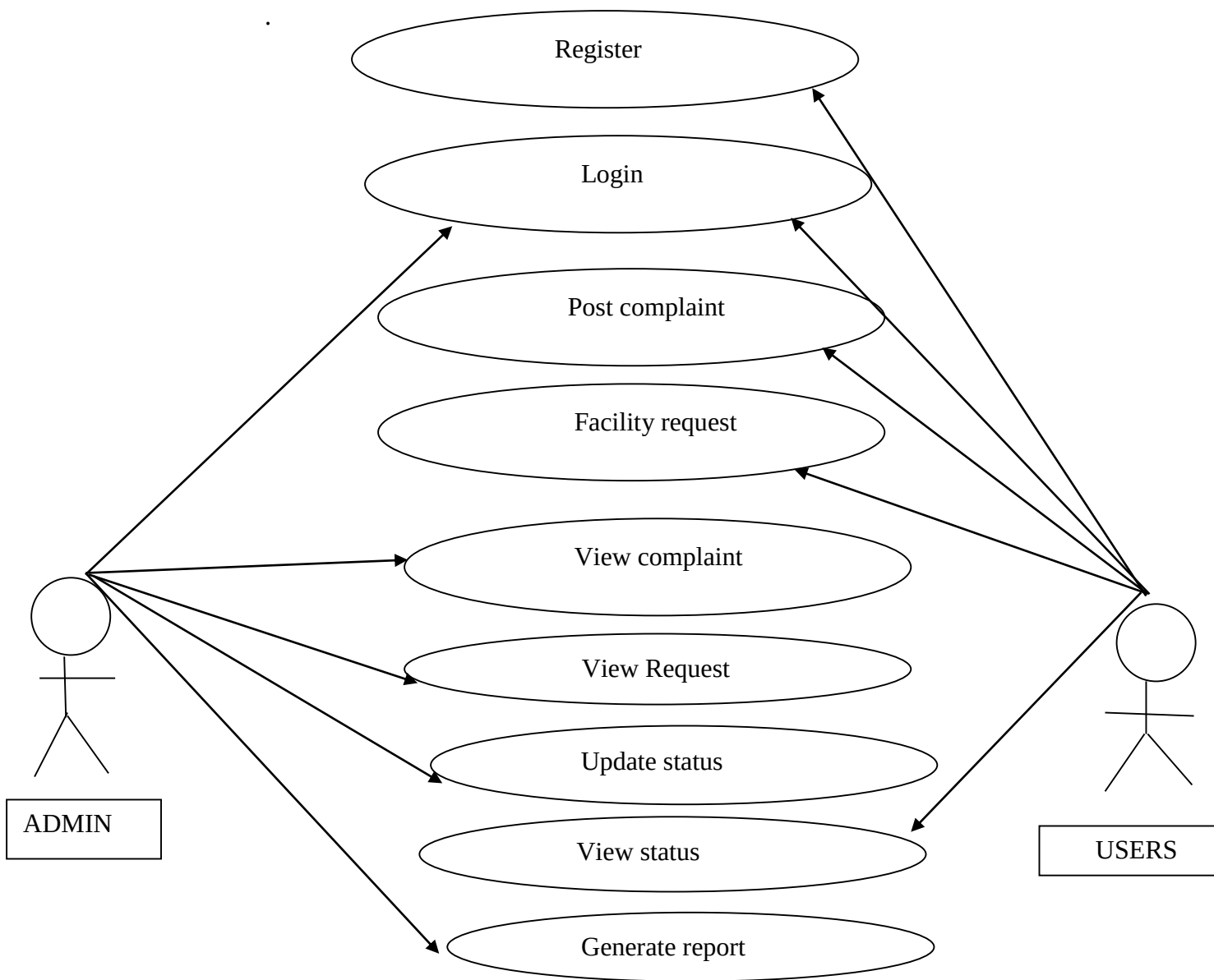
Fig.No.7.1.1Use case Diagram for Grievance Redressal system
