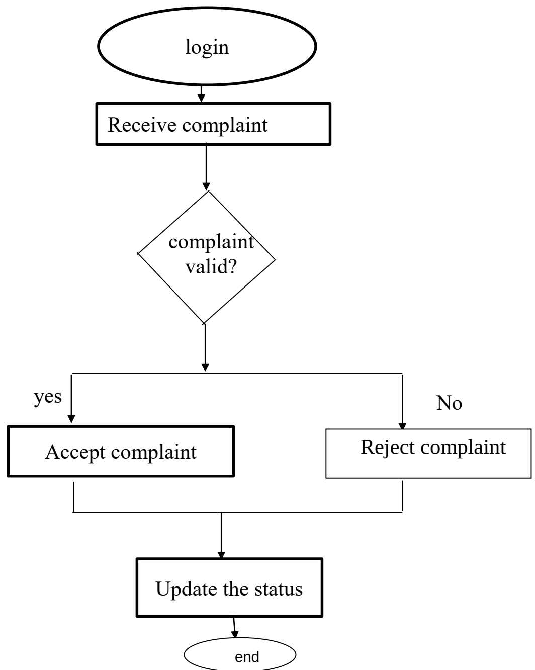
Fig.No. 7.1.3 Activity Diagram for Grievance redressal system
